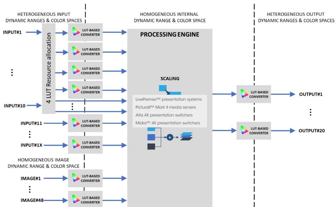
Figure 10: Dynamic Range et Color Space conversions in the Alta 4K series
