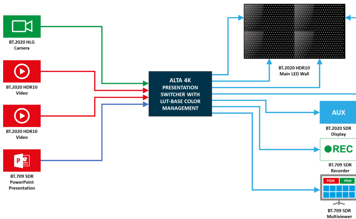
Figure 12: Example of heterogeneous workflow range setup with an Alta 4K system
