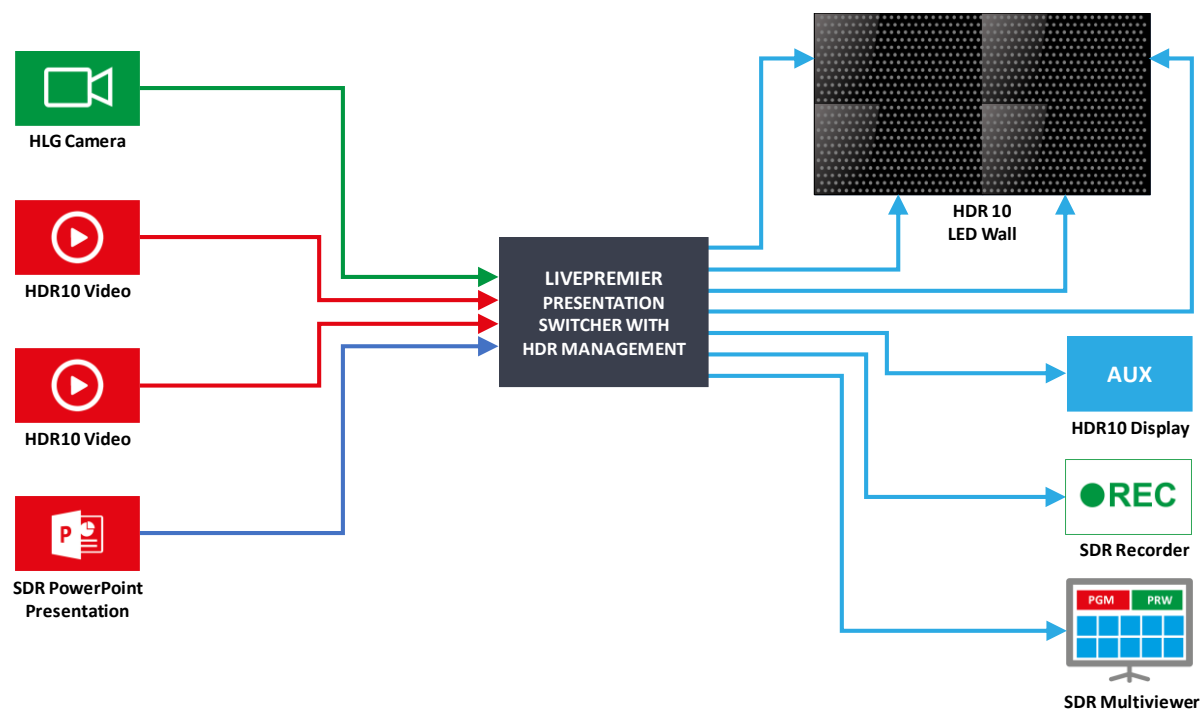
Figure 7: Example of heterogeneous HDR setup with Aquilon
