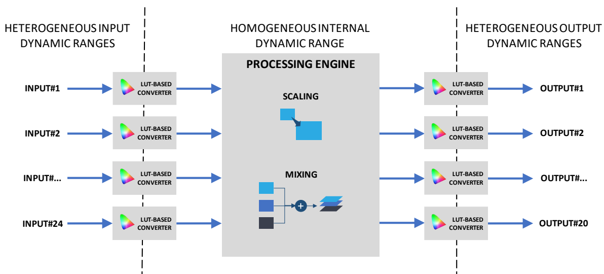
Figure 8: HDR conversions in Aquilon Series
