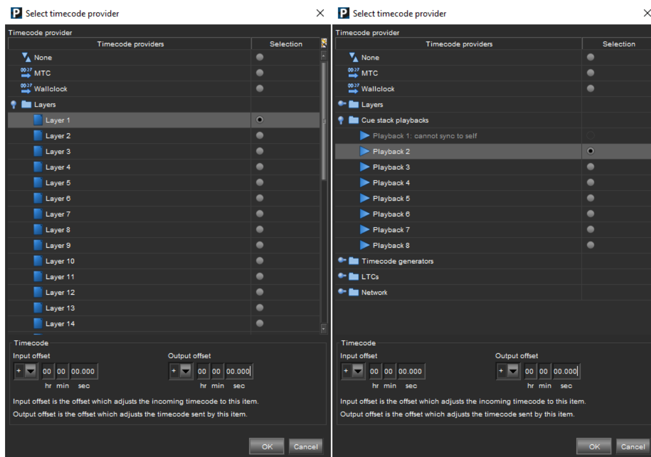
Fig. 85 - Selecting a Layer or a Playback as timecode provider
