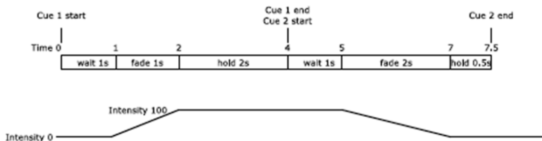
Fig. 72 - Cue timing example
