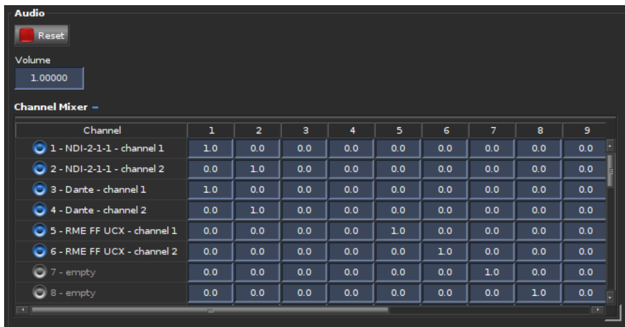
Fig. 69 - Commander Audio Channel Mixer
