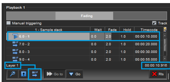
Fig. 82 - A cue triggered by selected timecode provider
