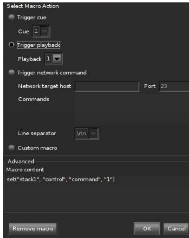
Fig. 95 - Entry macro for a cue start on start up
