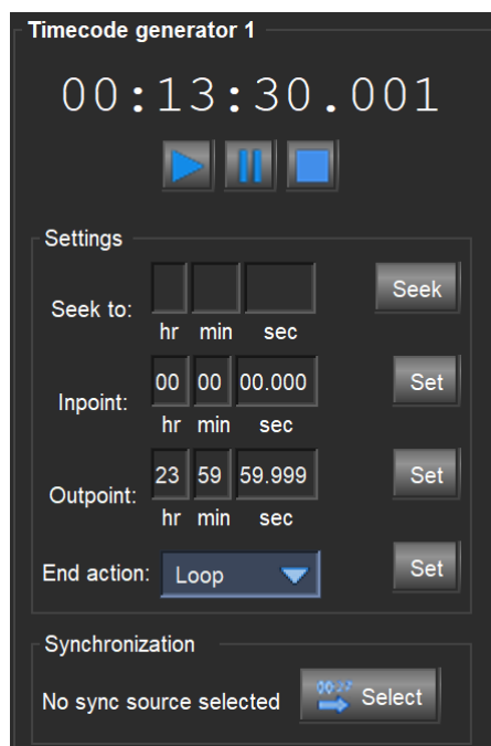
Fig. 87 - Timecode generator settings
